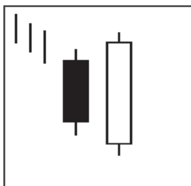
Bullish engulfing
