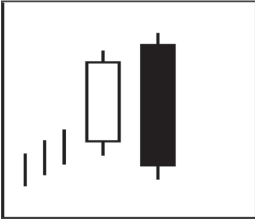
Bearish Engulfing
