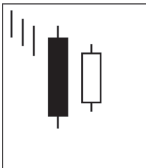
Bullish Harami
